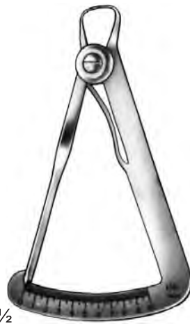
Iwanson 968-09-12 12 cm / 4 3/4" Decimal spring caliper Measuring capacity 0-10 mm
